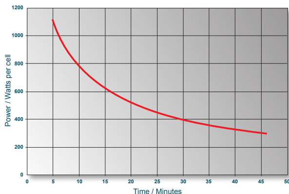
NSB12-590FT Discharge Curve to 1.67 vpc
