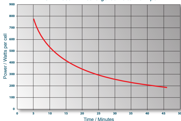
NSB12-380FT Discharge Curve to 1.67 vpc
